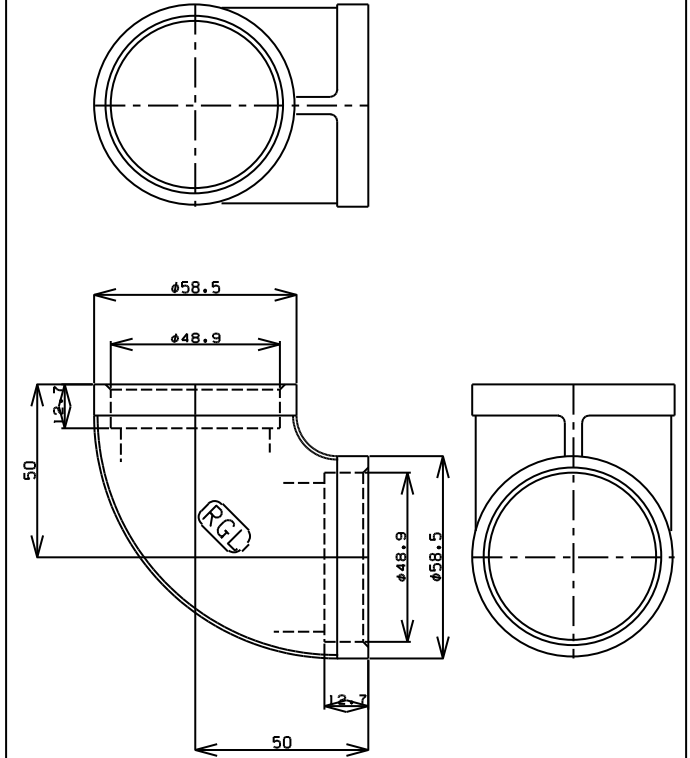
TITLE 溶接用90°エルボ MODEL R-1B-1-1/2
