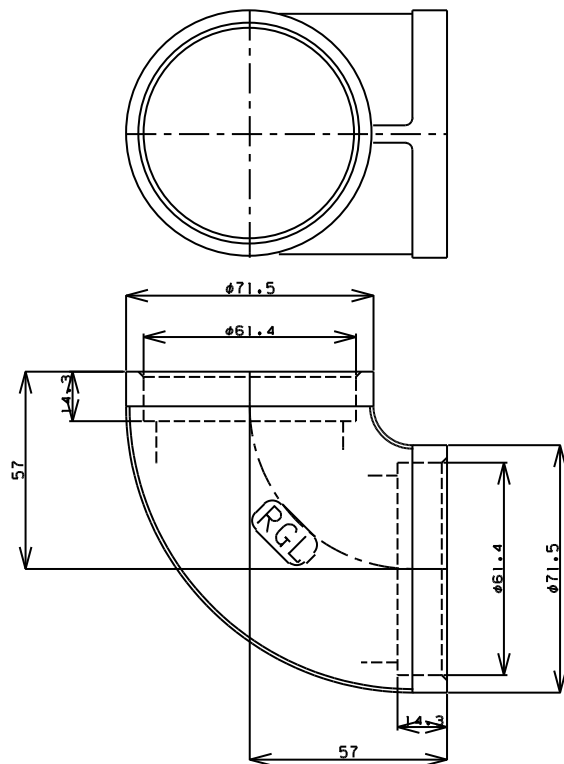
TITLE 溶接用90°エルボ MODEL R-1B-3/4
