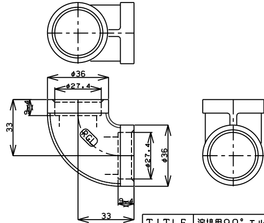
TITLE 溶接用90°エルボ MODEL R-1B-3/4
